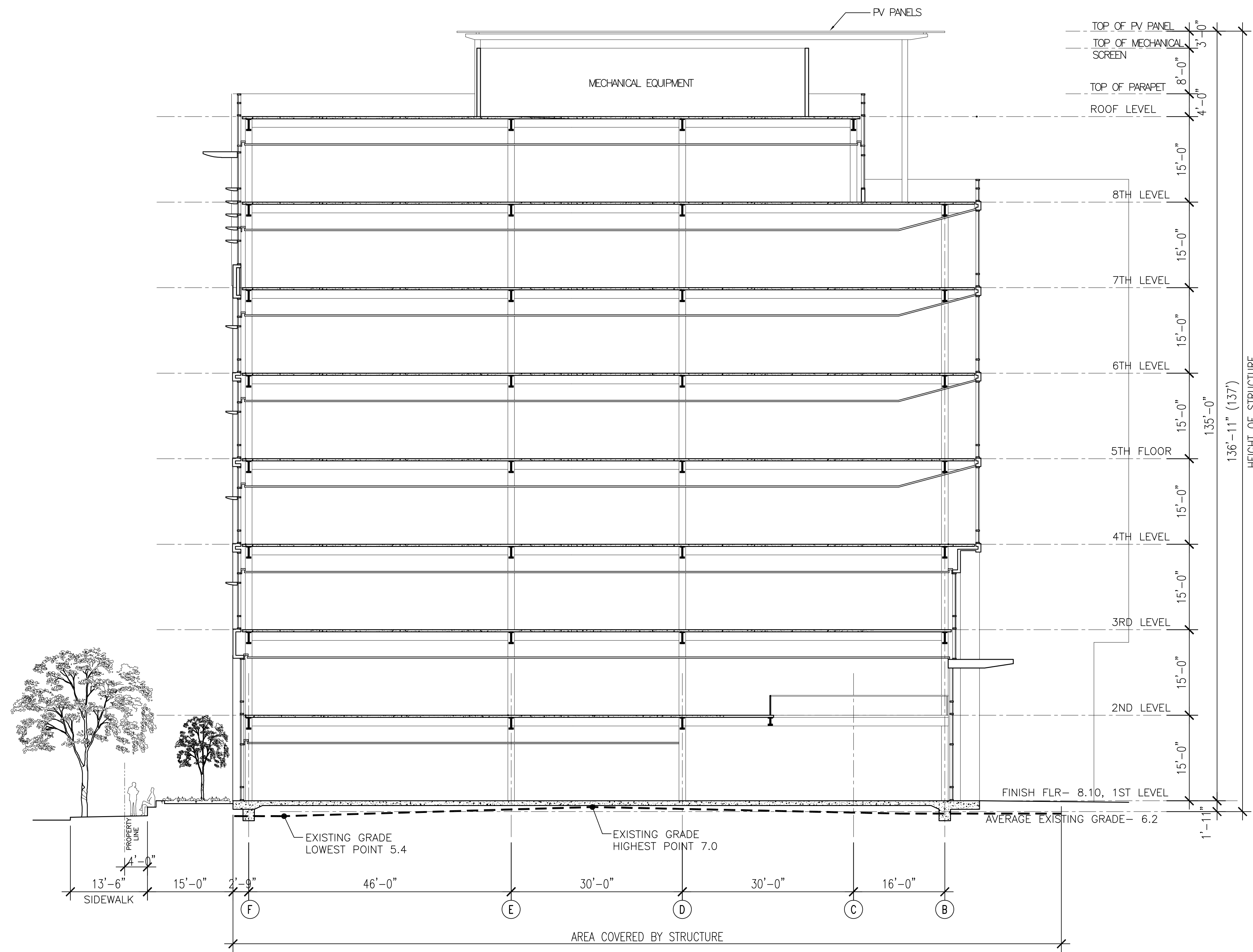
OFFICE BUILDING 2- SECTION
