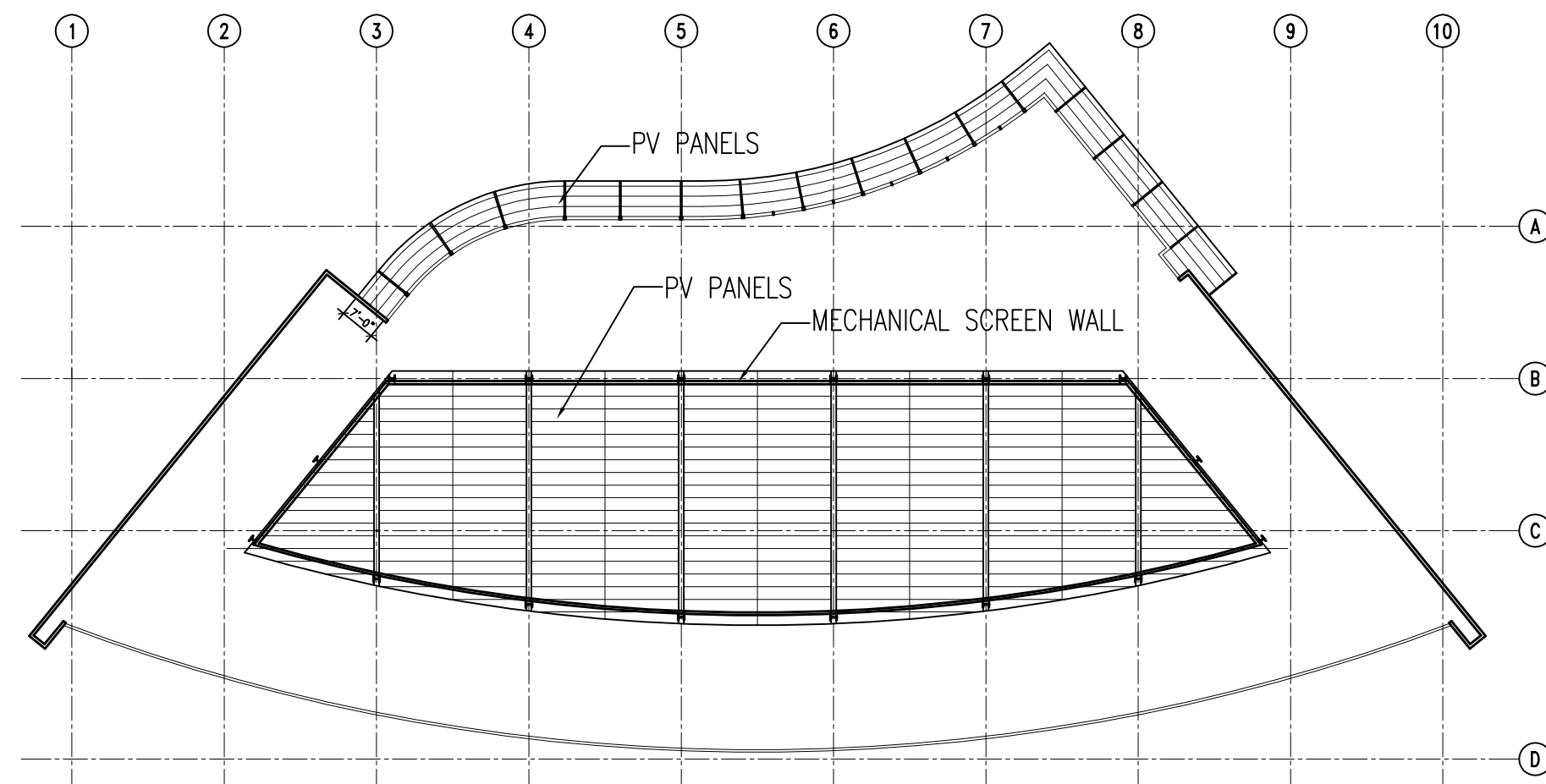
ROOF PLAN
