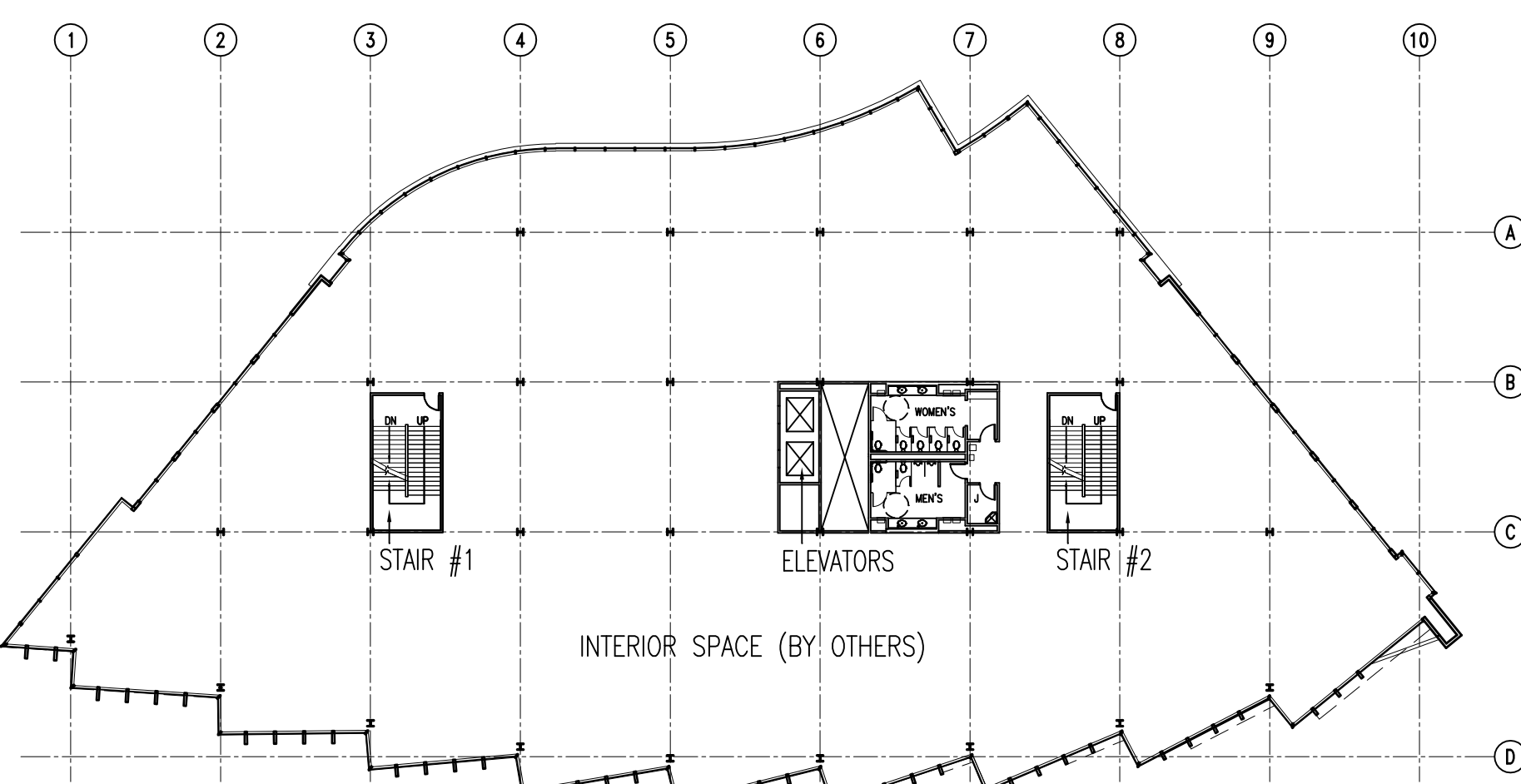
TYPICAL: 4TH~ 7TH FLOOR PLAN
